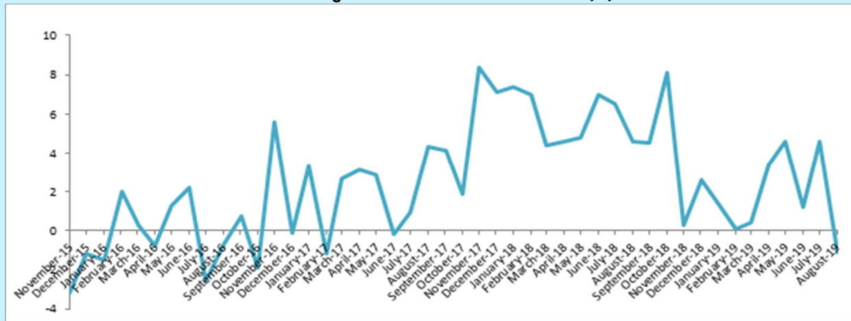
Trend in IIP growth (%)
